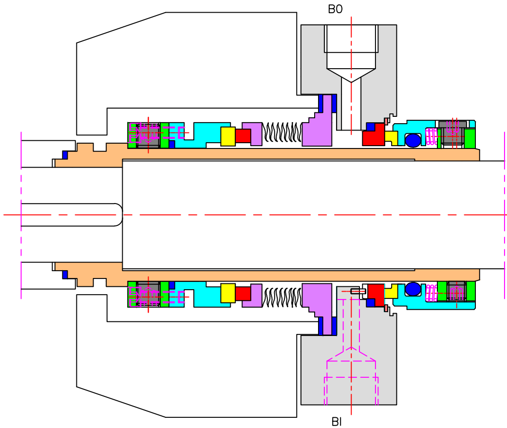
90 SERIES MULTI SPRINGS MECHANICAL SEAL TYPE M4452/9201 DOUBLE MECHANICAL SEAL ARRANGEMENT WITH DIFFERENT API PLAN 52
